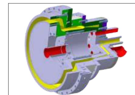
■ SINGLE-LAYER MOLD
